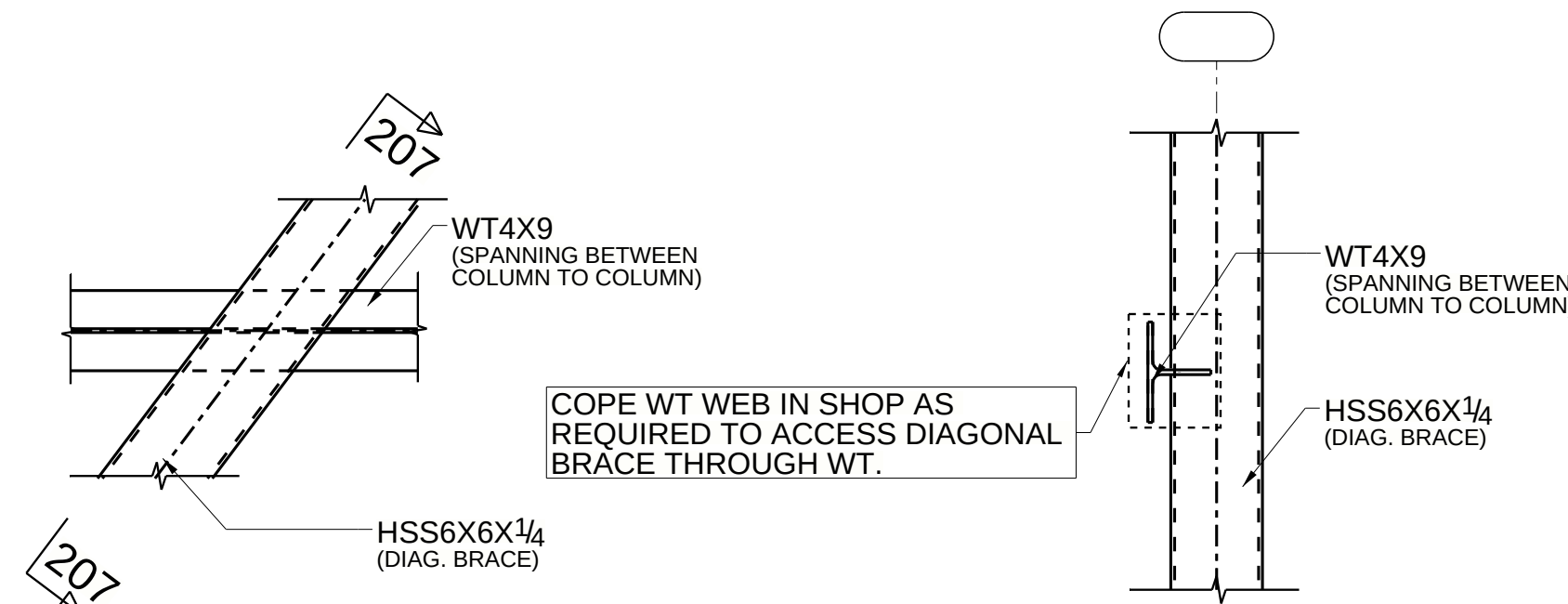
DETAIL 206
