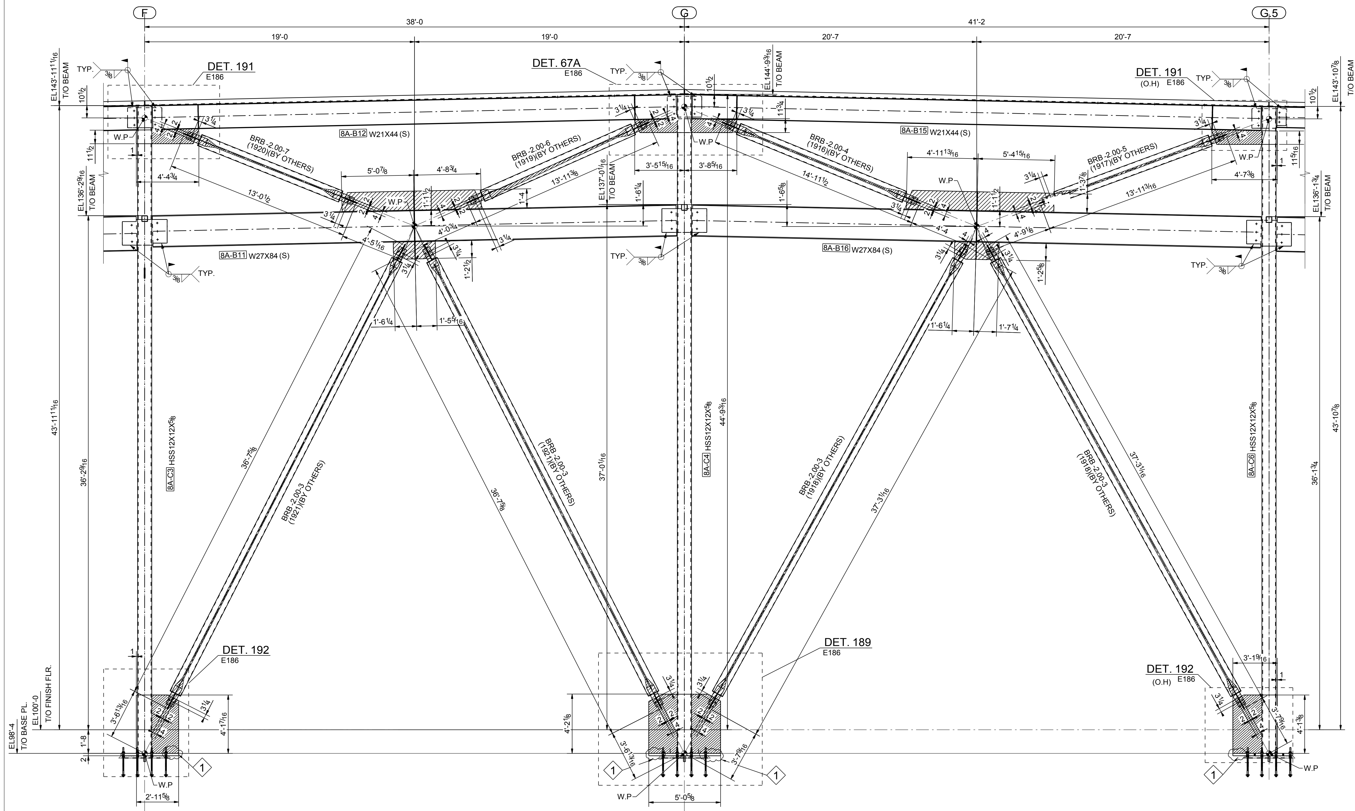
SECTION 67 - 67 E128 BRACED FRAME ELEVATION ALONG GRID "17"
