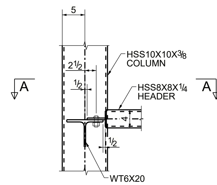
DETAIL 4A
