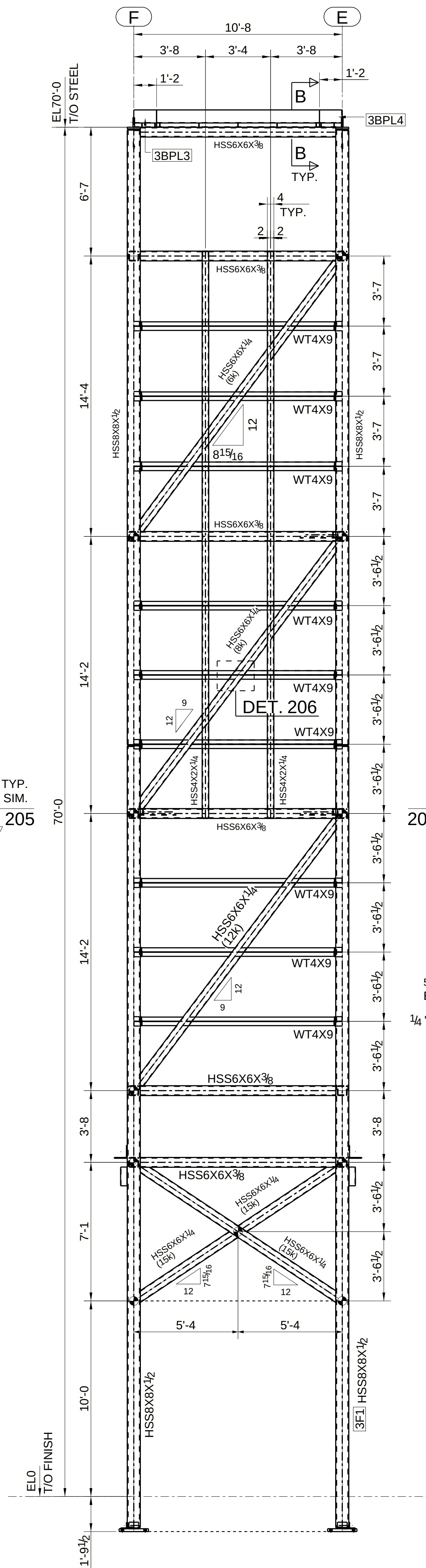
SECTION 204 - 204
