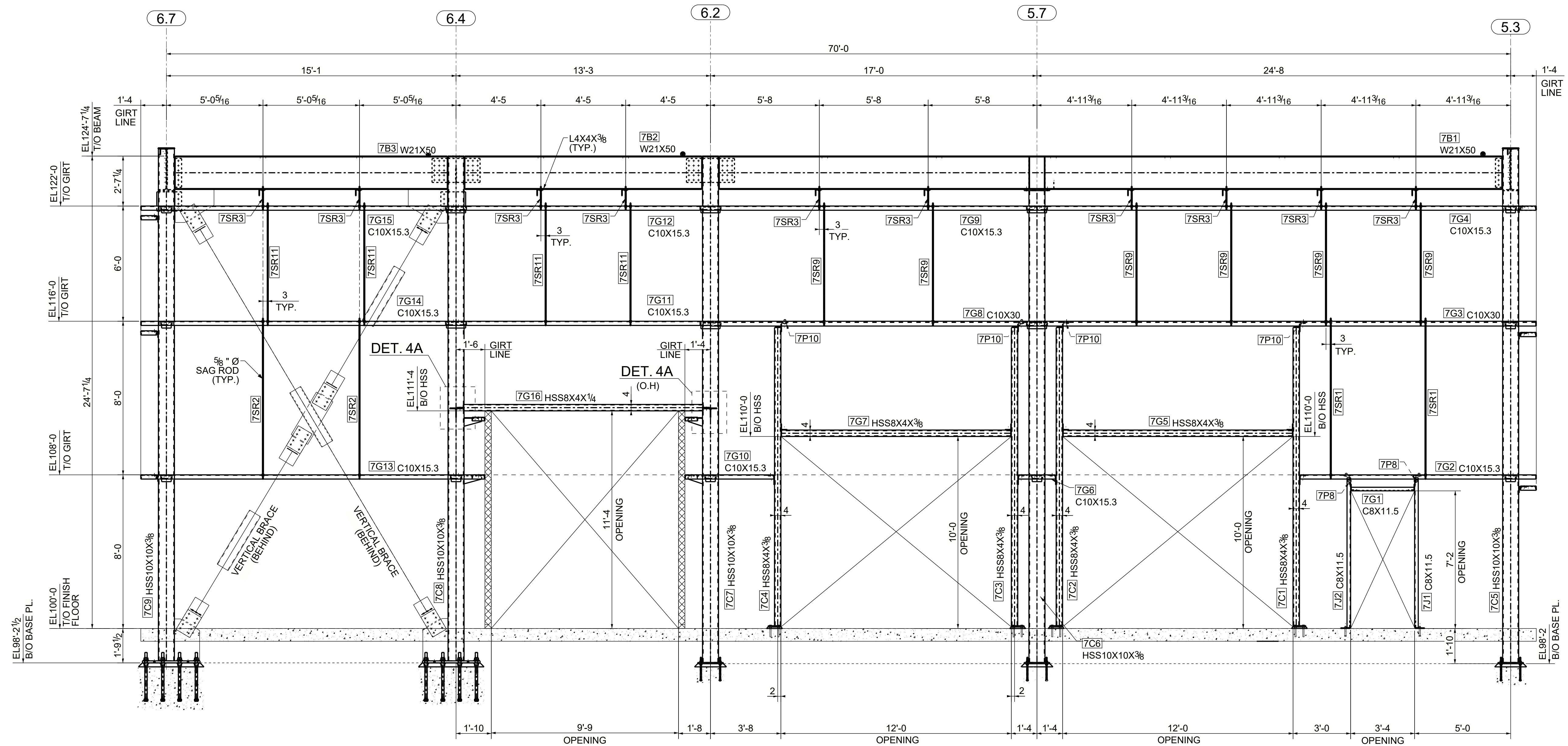
SECTION 4 - 4 E701 GIRT ELEVATION ALONG GRIDLINE - A1 (REFER ELEVATION : 6/66-88.S.03.01.)
