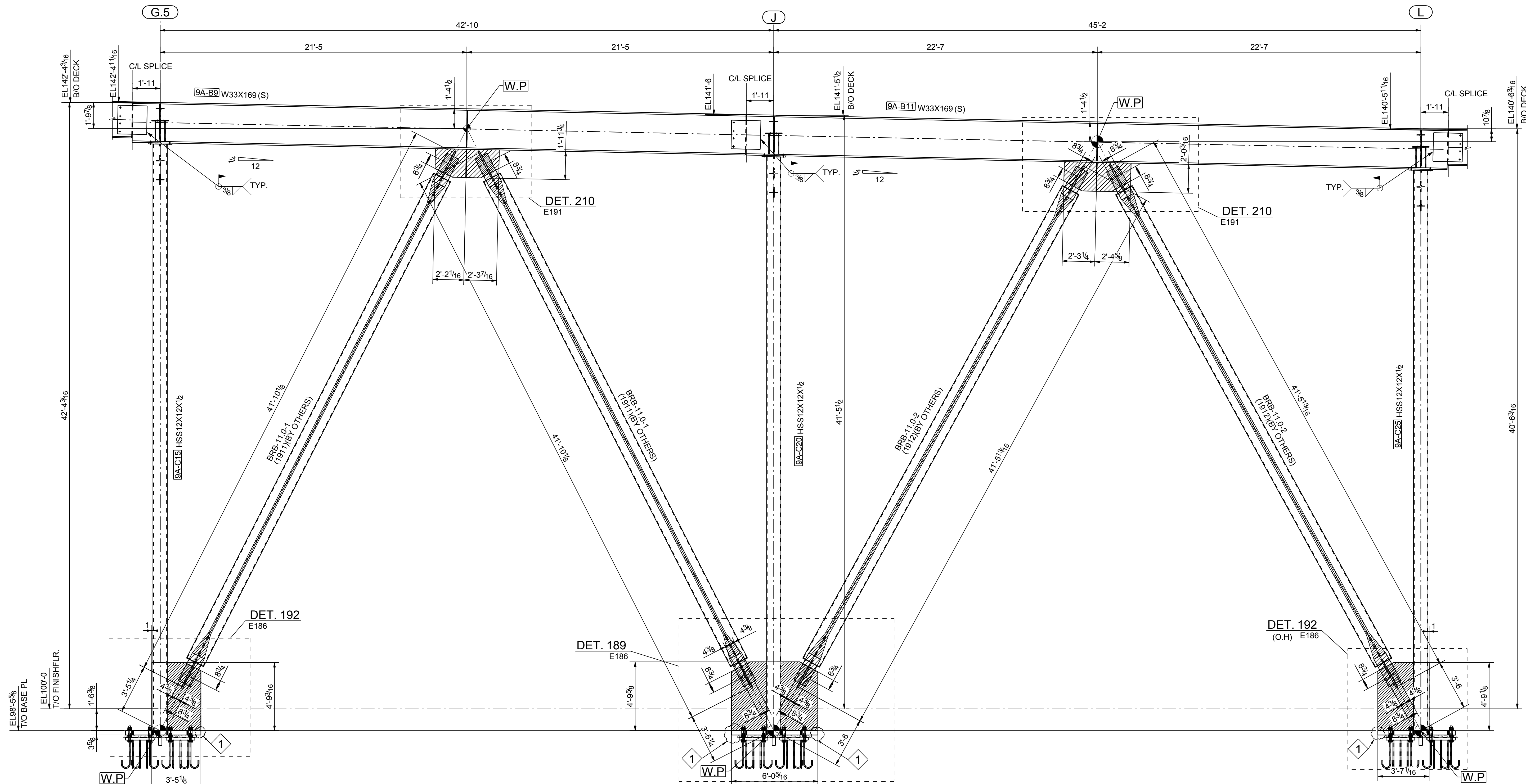
SECTION 80 - 80 E133 BRACED FRAME ELEVATION ALONG "24" (REFER :BRACED FRAME ELEVATION ALONG GRID "24" (S-302))
