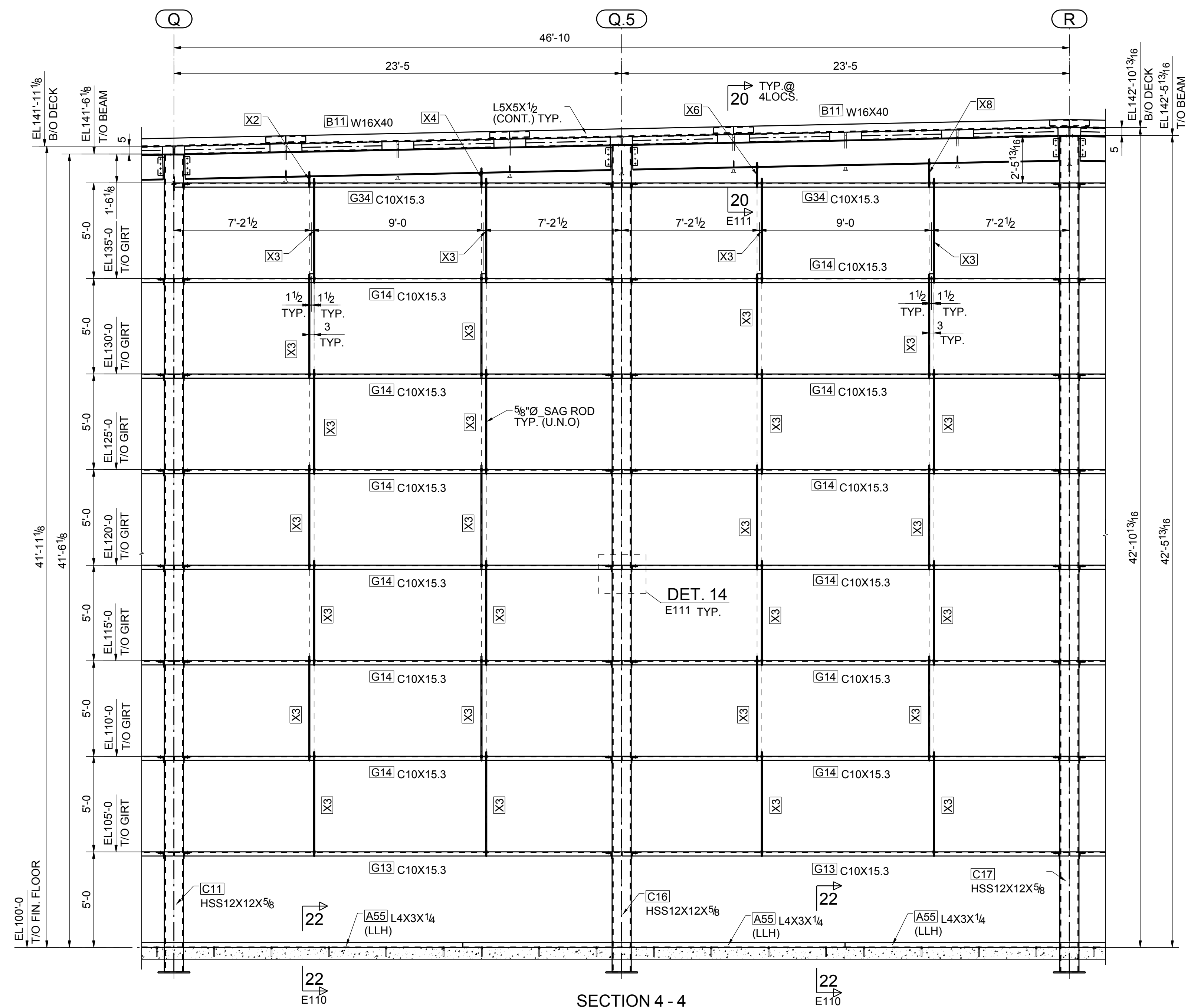
SECTION 4 - 4 E102 WIND GIRT ELEVATION @ ALONG GRIDLINE "20" (REFER : WIND GIRT ELEVATION @ GRID "20" / S-301) SEQUENCE - 1
